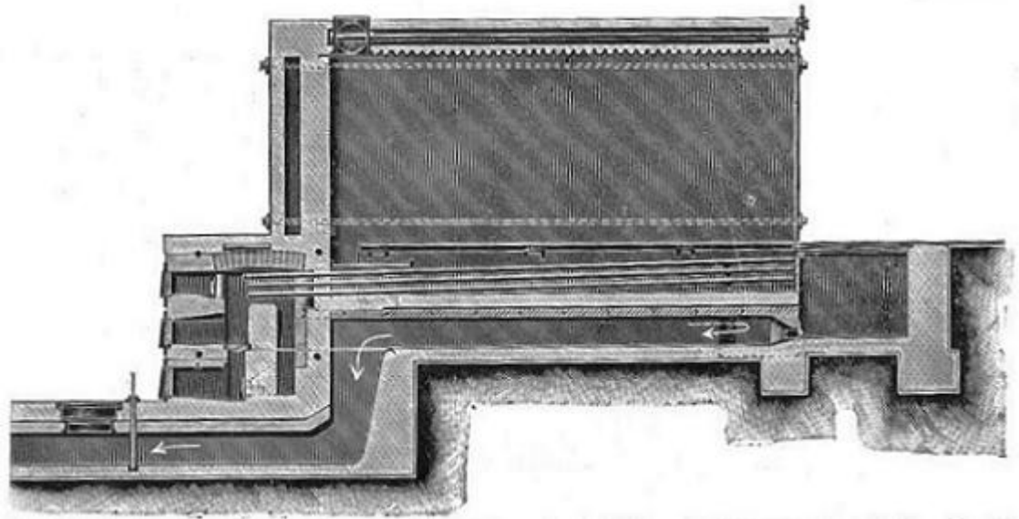
FIG. 8.—Japanning and Enamelling Oven Heated by Single Hot-water Pipes sealed at both ends with Furnace in Rear.
